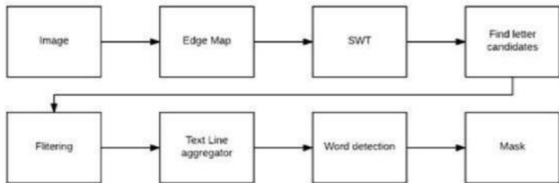
Figure 6 Stroke Width Algorithm Flowchart
